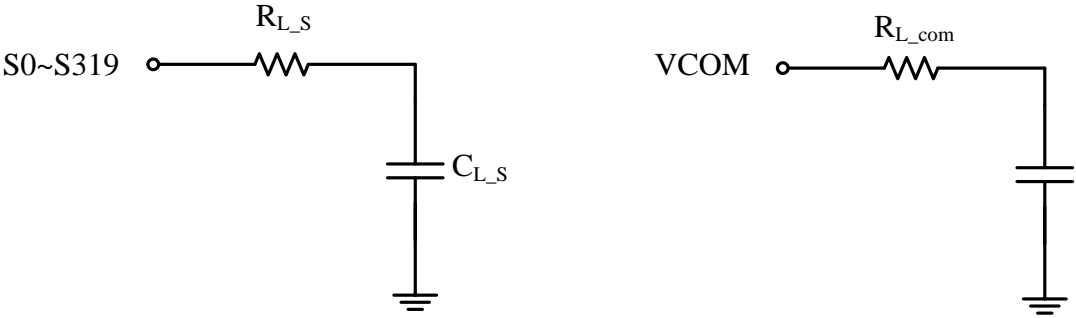
Figure 9: RC loading
